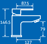
Nero Basin Mono 3 0.2 bar min. – Including click clack waste 12778 £125
