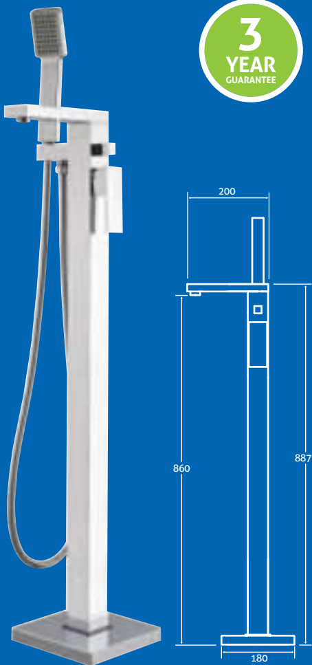
Nero Floor Standing Bath Shower Mixer 1.0 bar min. 34293 £460
