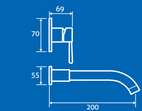
Trajan Wall Mounted Basin Mixer 0.2 bar min. 69906 £142
