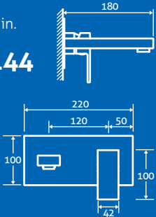
Nero Bath Filler 3 0.3 bar min. 12779 £202
