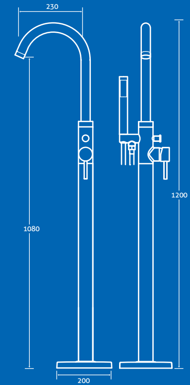
Trajan Floor Standing Bath Shower Mixer 1.0 bar min. 12786 £406
