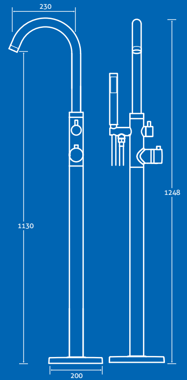
Trajan Floor Standing Thermostatic Bath Shower Mixer 1.0 bar min. 34291 £460
