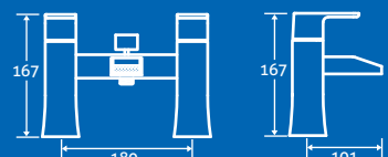
Zest Waterfall Bath Shower Mixer 3 0.5 bar min. – Including handset, hose and bracket. 12790 £305
