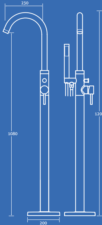
Trajan Floor Standing Bath Shower Mixer
